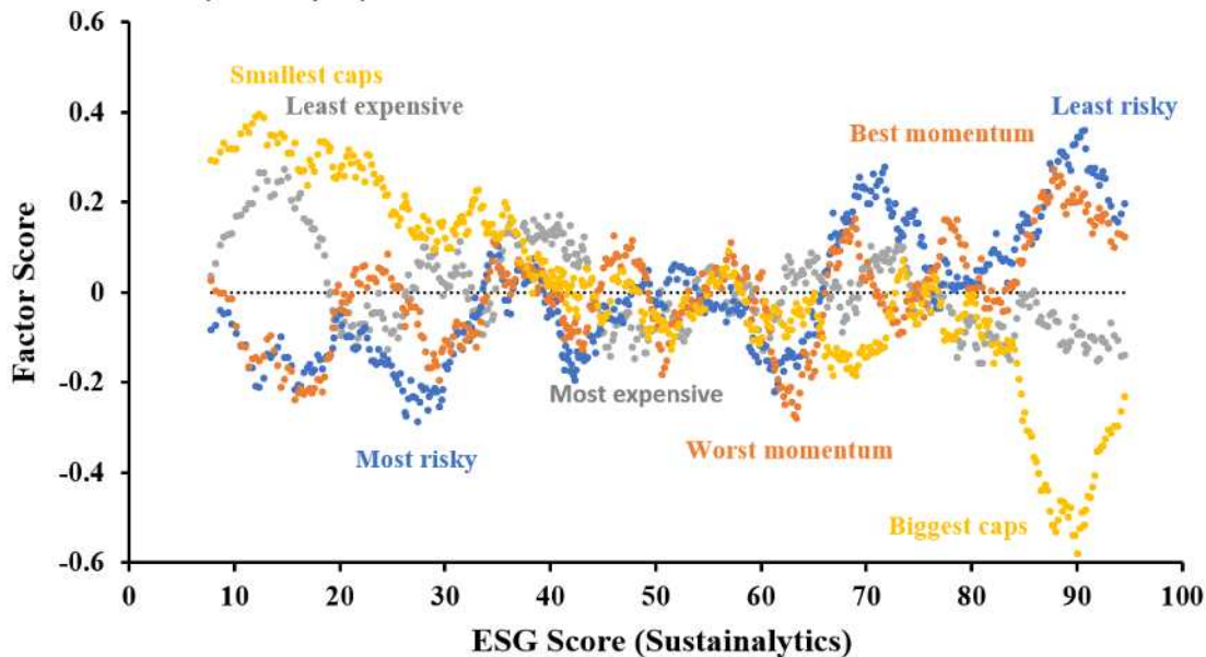
Exhibit 1: ESG score (Sustainalytics) vs. factorial score for stocks in the S&P500 index at the end of 2020
