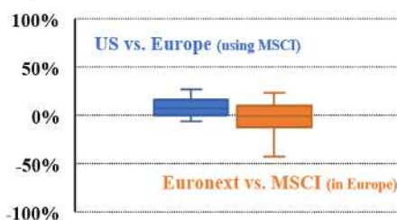
Exhibit 5: Correlations of ESG investments between regions and providers
