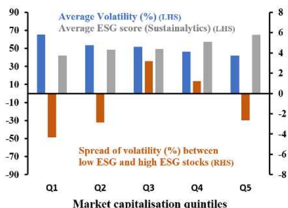
Exhibit 2: ESG score (Sustainalytics) vs. low volatility for S&P500 stocks
